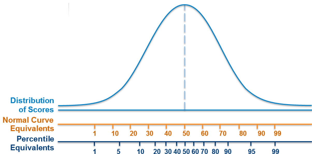
Figure 2: Distribution of Achievement: Scores, NCEs and Percentile Rankings
